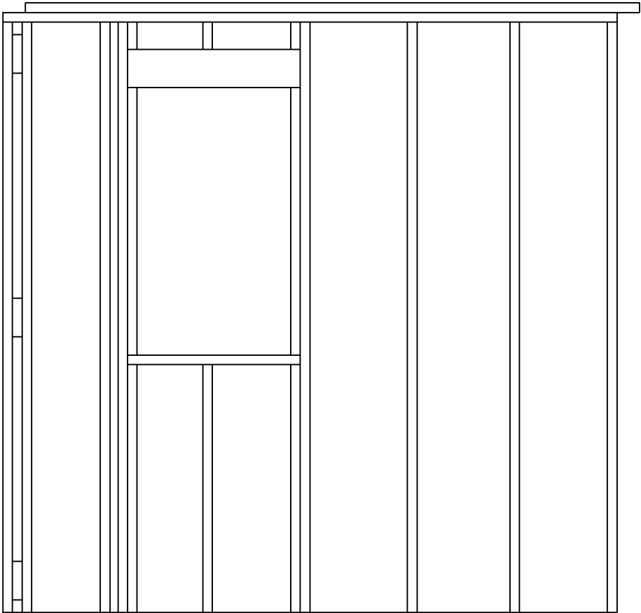
FRAMING ELEVATION
